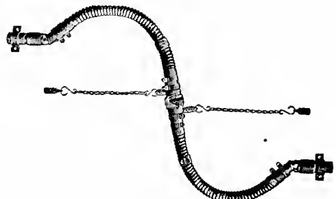
Fig. 2989. THE McELROY STEAM-HOSE COUPLING.
